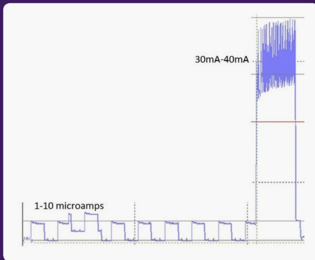
Figure 14. The power consumption of a device at 1-10 micro-amps while in hibernation mode and at 30-40 milli-amps while in active mode.
