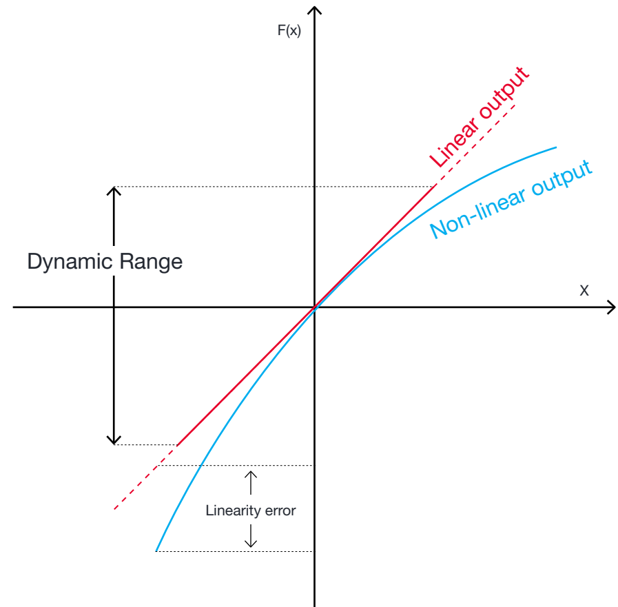
Figure 6. Dynamic range and linearity of sensors
