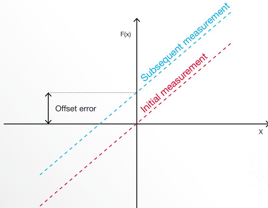
Figure 18. Offset error affecting measurement accuracy
