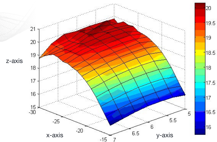
Figure 16. Example of a three-dimensional plot of a characterized sensor. The Z-axis represents the sensor's readout, such as voltage, power, temperature, or force. The X and Y axis are the external conditions the sensor is subjected to, such as input frequency, operating temperature, or pressure.
