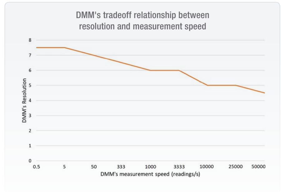
Figure 11. Graph of DMM's resolution versus speed
