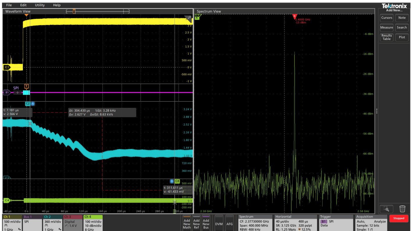
FIGURE 14. We are triggering on the SPI bus command that tells the VCO what frequency to tune to. In this case, it's 2.4 GHz. Using Spectrum Time, we were able to scroll through the acquisition and see when the RF output stabilized at 2.4 GHz. Then, using cursors, we can measure from the trigger event to Spectrum Time's location and see that it took 304 \mu s for the output to achieve the desired frequency.
