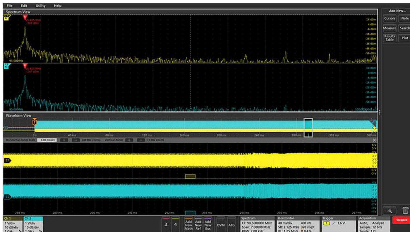
FIGURE 15. When debugging tasks demand it, multiple channels can be analyzed simultaneously. Here, two channels show the startup of a clock signal from two different points in a circuit.
